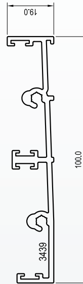
3439 SILL 2 TRACK LP
