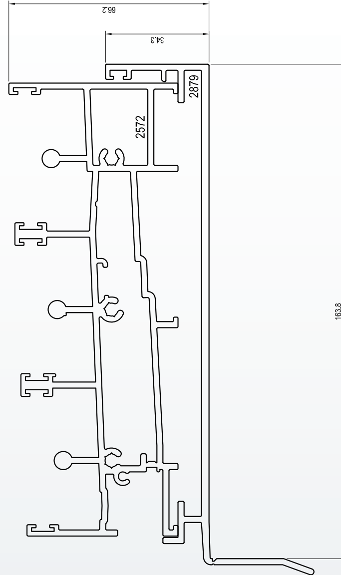
2572 SILL 3 TRACK STD WITH 2879 SUBSILL 'I' 150
