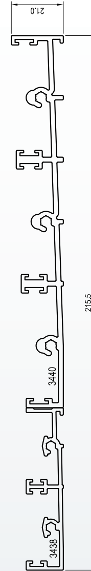
3440 SILL 3 TRACK LP WITH 3438 SILL PLANT-ON LP
