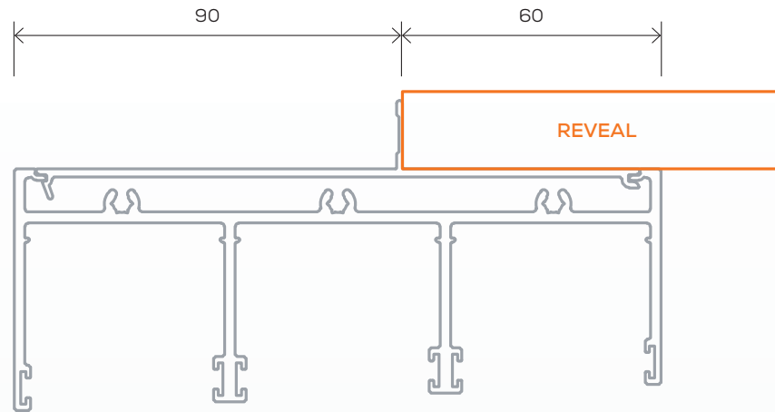
Commercial Sliding Door (150mm)
