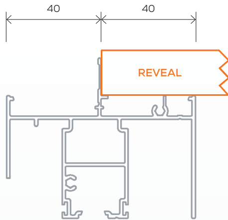
Essential Sliding Door (80mm)
