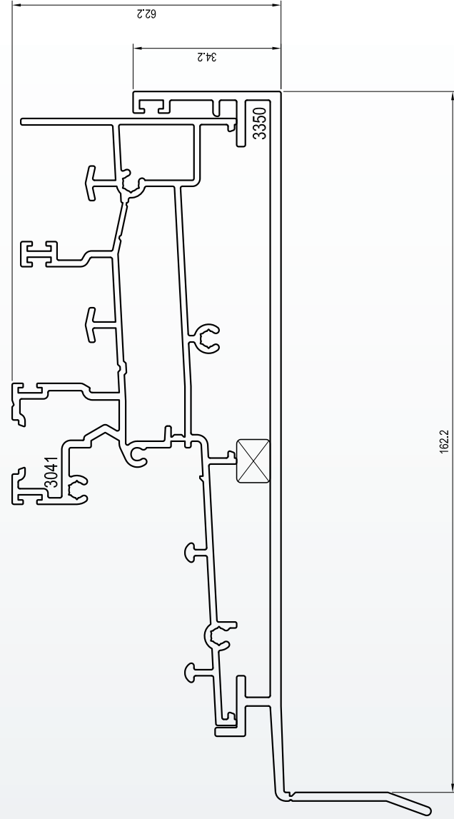
3041 SILL STACKER WITH 3350 SUBSILL '15' 140
