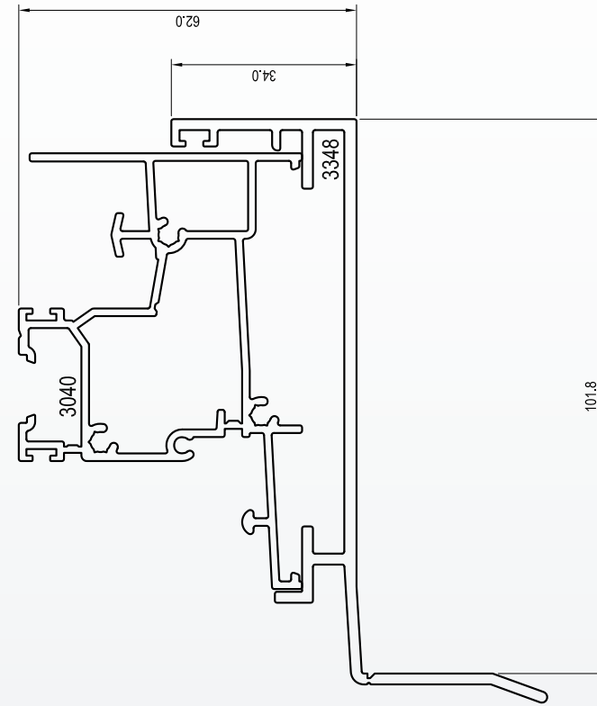
3040 SILL STD 80 WITH 3348 SUBSILL '15' 80
