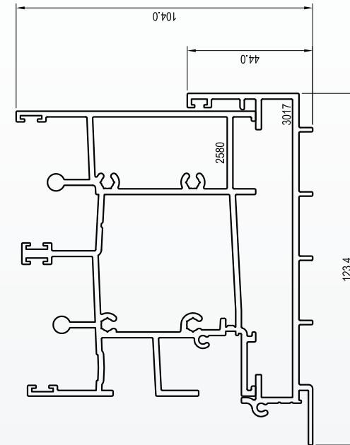
2580 SILL 2 TRACK HP WITH 3017 SUBSILL BAFFLED 100
