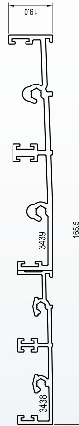
3439 SILL 2 TRACK LP WITH 3438 SILL PLANT-ON LP
