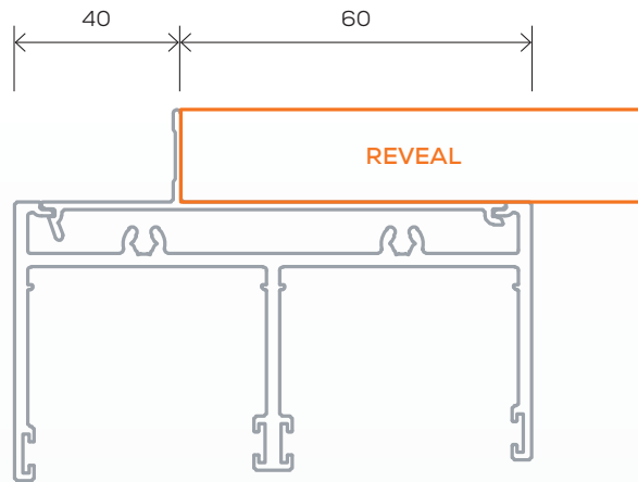
Commercial Sliding Door (100mm)
