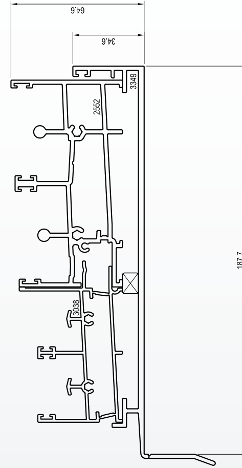
2552 SILL 2 TRACK STD & 3038 SILL PLANT-ON WITH 3349 SUBSILL '15' 166
