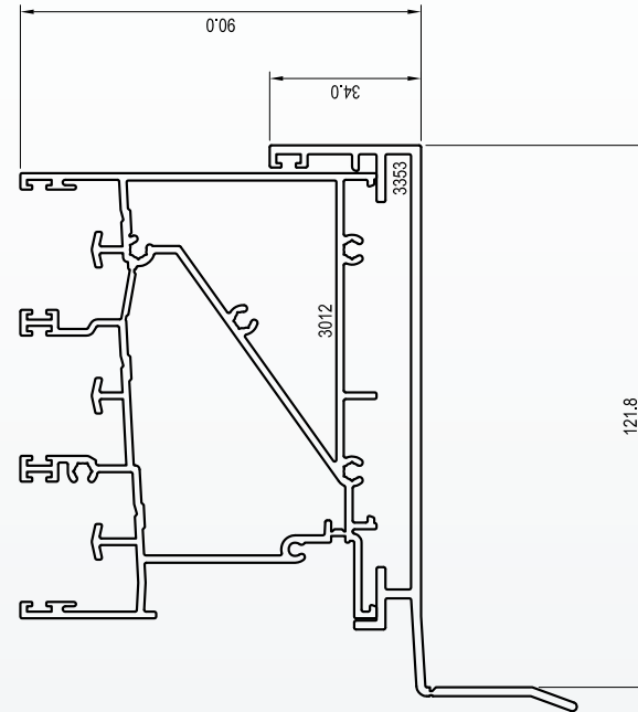
3012 SILL 3 TRACK 600Pa WITH 3353 SUBSILL '15' 100
