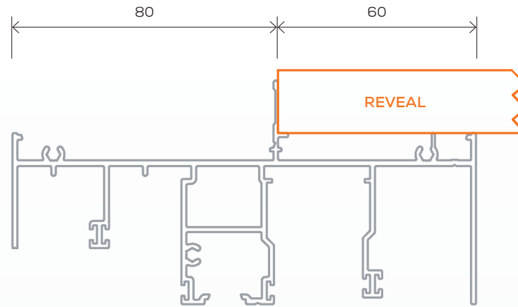
Essential Sliding Door (140mm)
