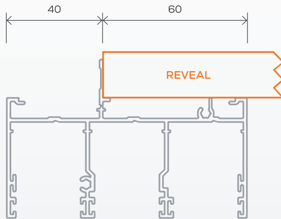
Signature Sliding Door (100mm)
