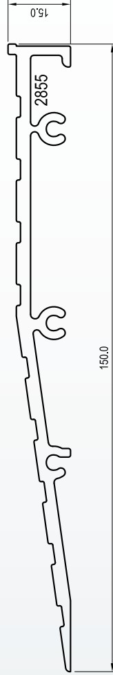
2855 THRESHOLD DISABLED 150 WITH 3017 SUBSILL BAFFLED 100
