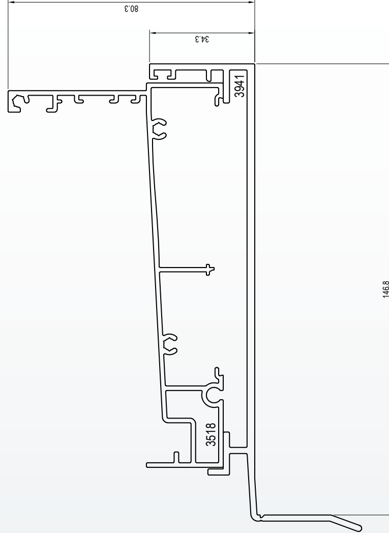
3518 SILL LOUVRE 125 WITH 3941 SUBSILL '15' 125
