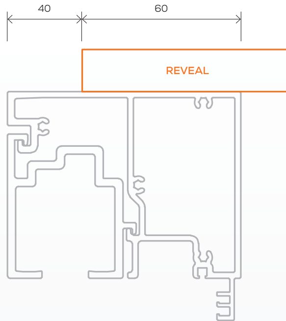
Commercial Bi-fold Window (100mm)
